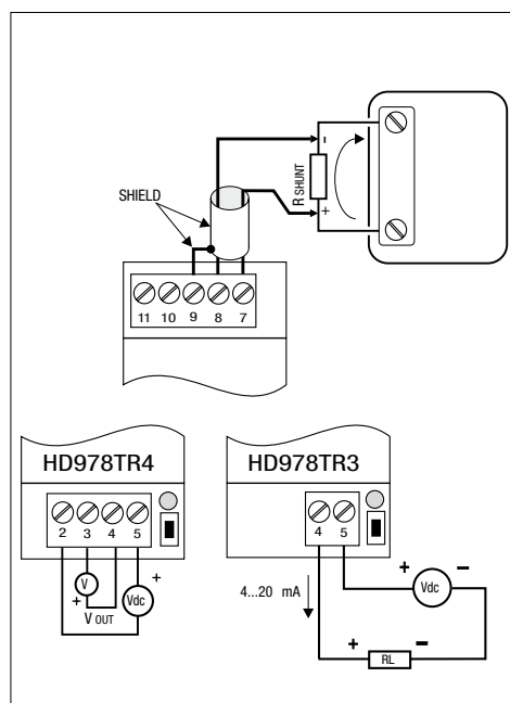
Fig.7 Connection diagram of HD978TR3 and HD978TR4 to a SHUNT.
