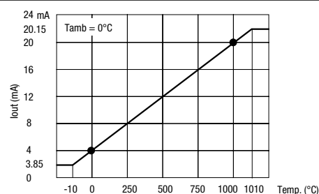
Fig. 2 0... 1000°C current output according to temperature
