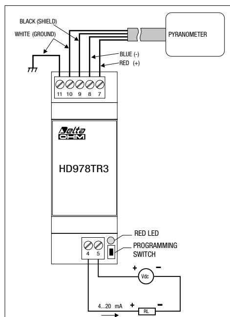
Fig.5 Connection diagram of HD 978TR3 to a pyranometer.
