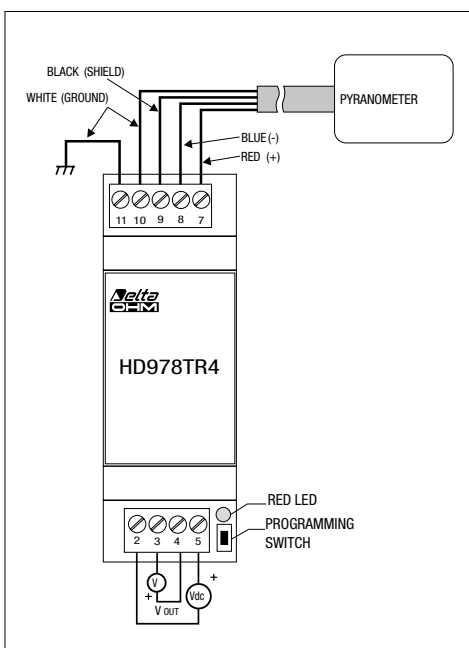
Fig.6 Connection diagram of HD978TR4 to a pyranometer
