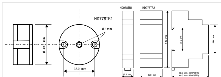
Fig.1 Mechanical dimensions.
